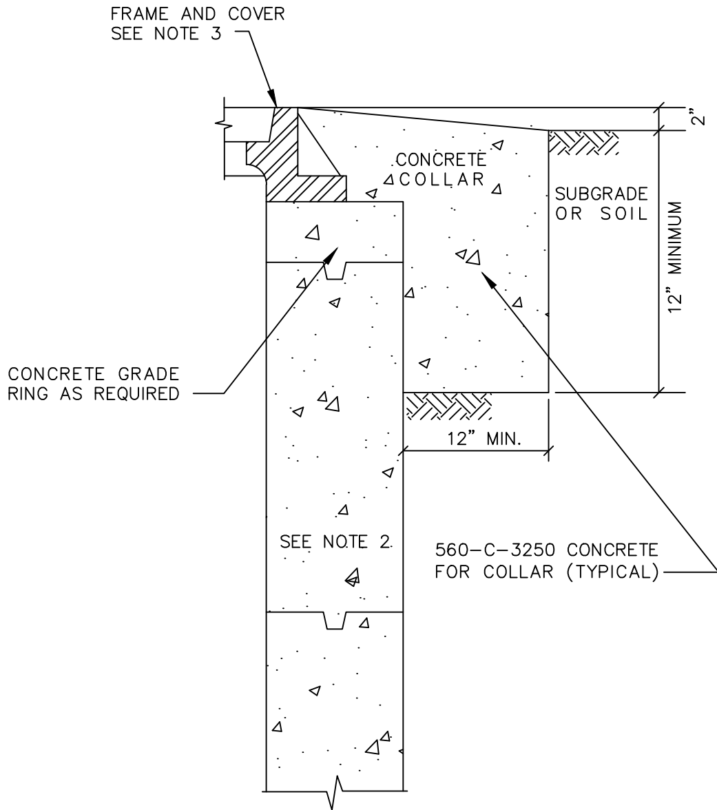
TYPE 'C' FOR UNPAVED TRAVELED WAYS
