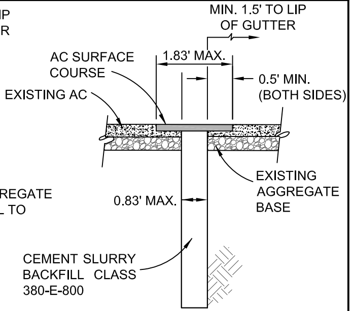
TYPE B ROCKSAW TRENCH (SEE SRF-08B FOR TRENCH PAVING NOTES)
