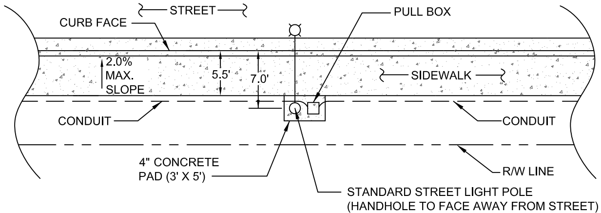
CASE 2: TYPICAL 5' WIDE SIDEWALK
