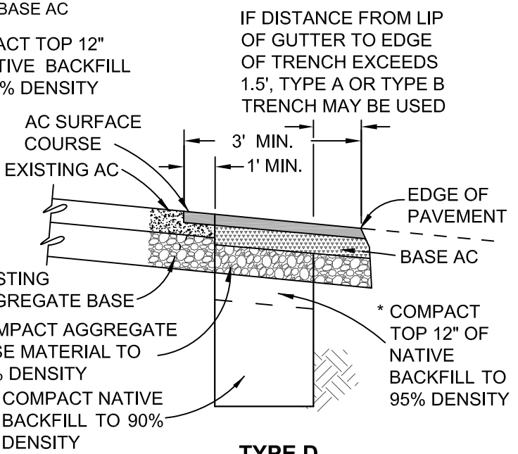
TYPE D TRENCH AT EDGE OF PAVEMENT (SEE SRF-08B FOR TRENCH PAVING NOTES)
