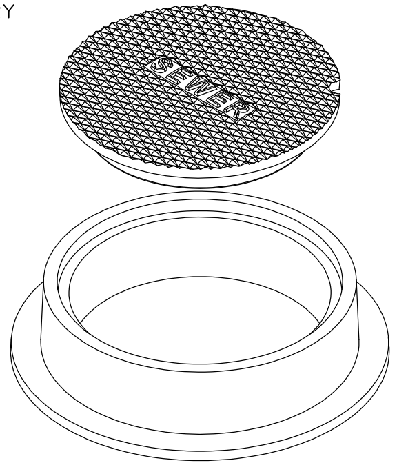
ISOMETRIC VIEW
