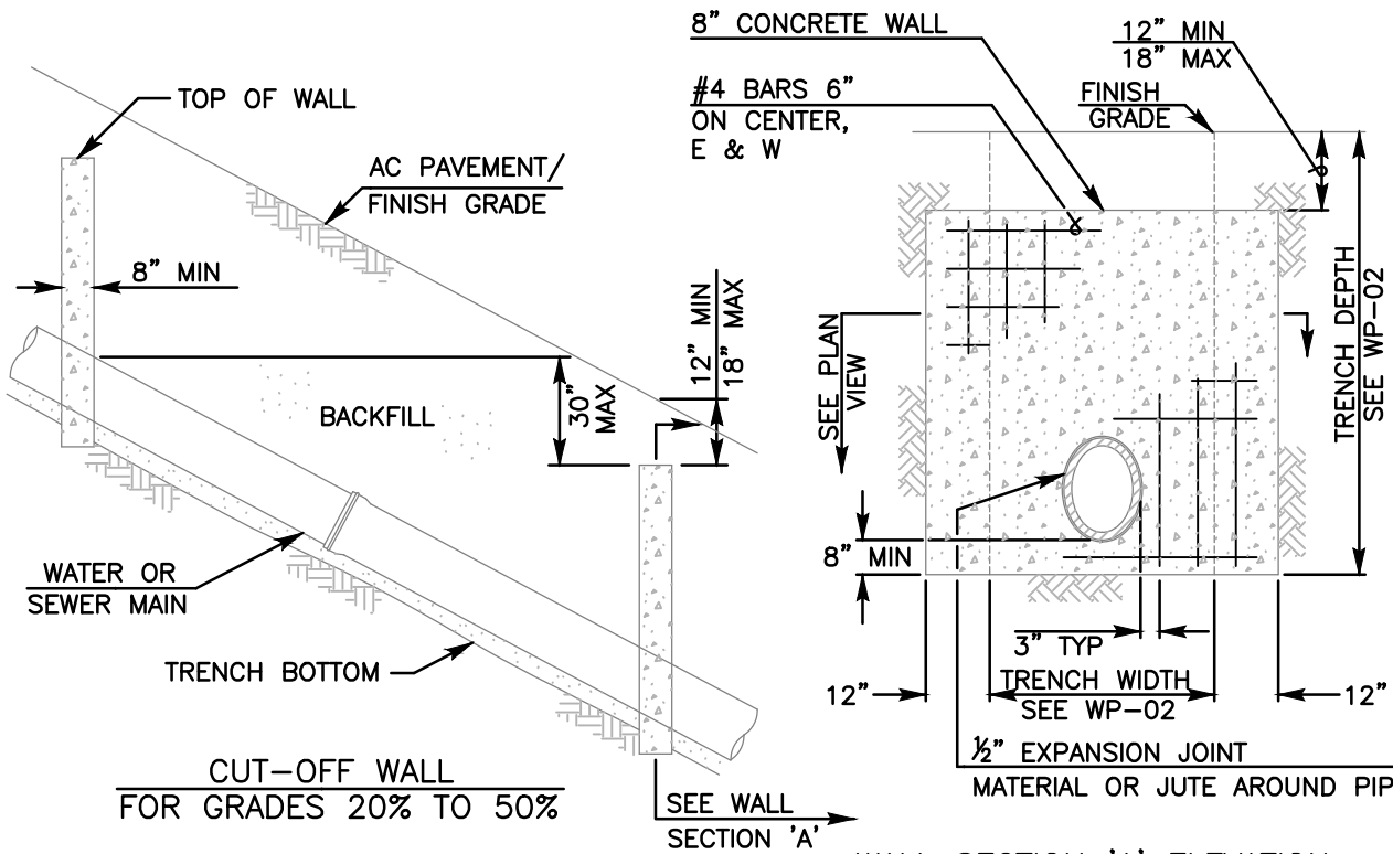
WALL SECTION 'A' ELEVATION
