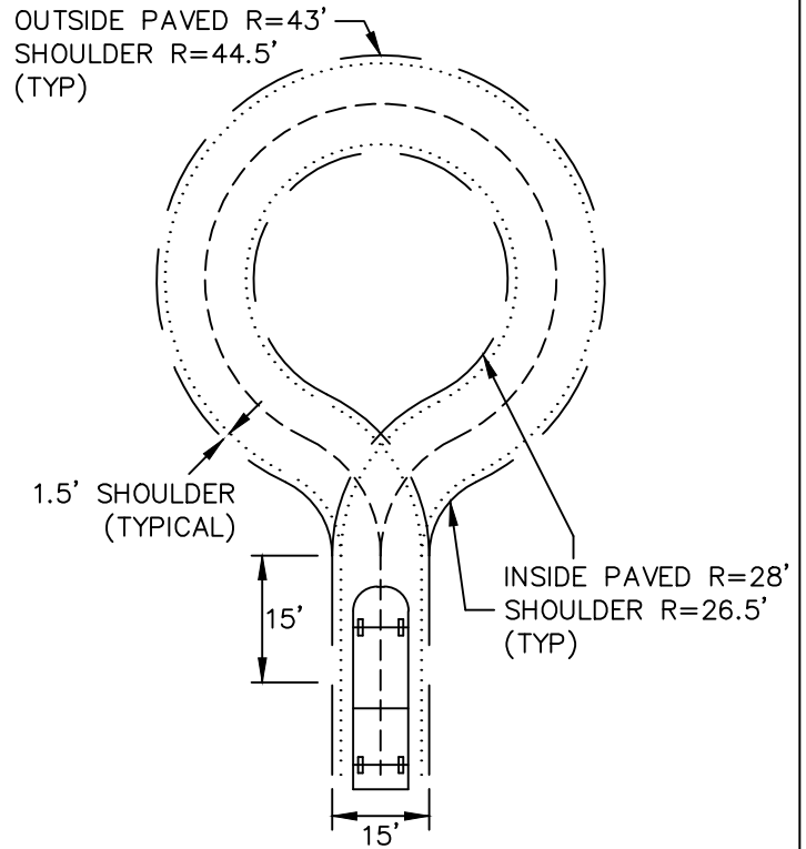
TYPE 2: CUL-DE-SAC TURN AROUND
