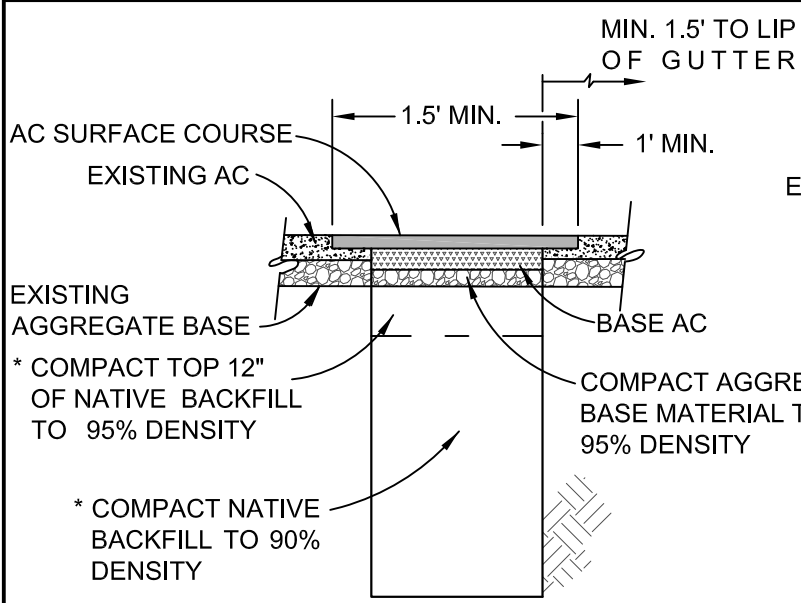
TYPE A EXCAVATED TRENCH (SEE SRF-08B FOR TRENCH PAVING NOTES)
