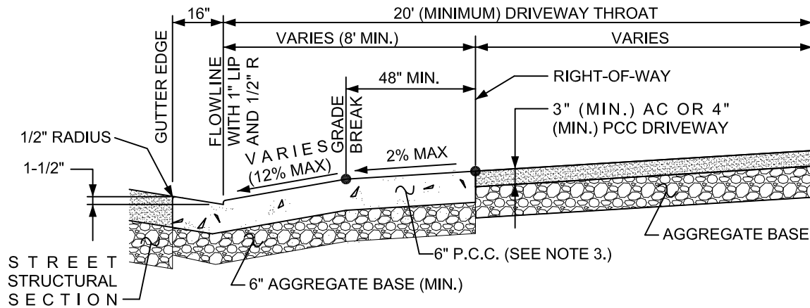
CENTERLINE CROSS SECTION
