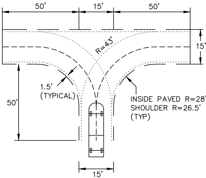
TYPE 3: HAMMERHEAD "T" TURN AROUND
