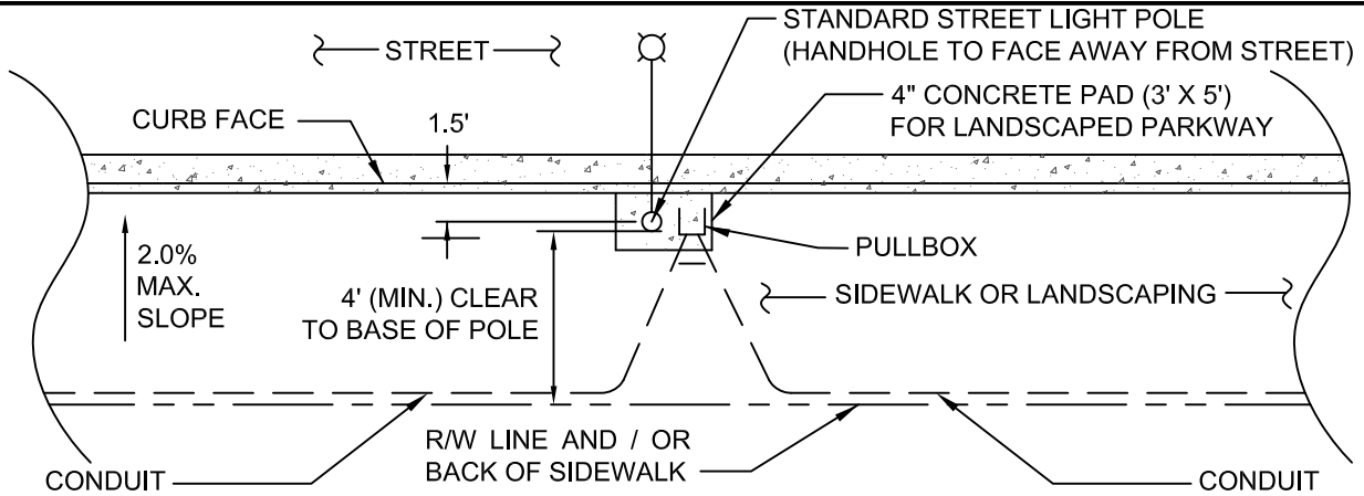
CASE 1: FULL WIDTH SIDEWALK OR NO SIDEWALK
