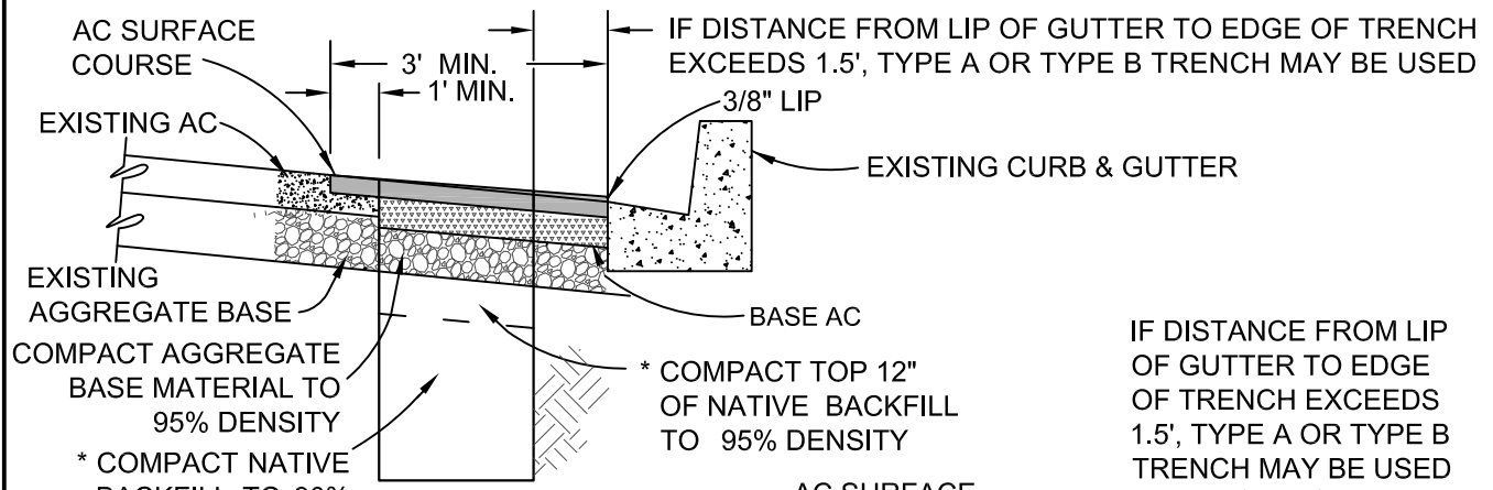
TYPE C TRENCH ADJACENT TO GUTTER (ROCKSAW OR EXCAVATED) (SEE SRF-08B FOR TRENCH PAVING NOTES)
