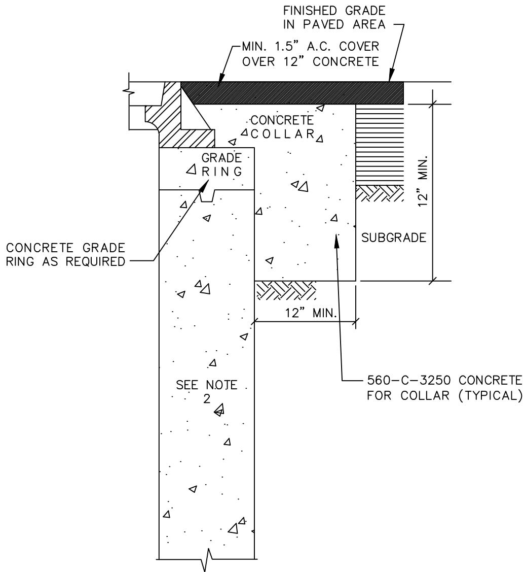
TYPE 'B' FOR PAVED AREAS
