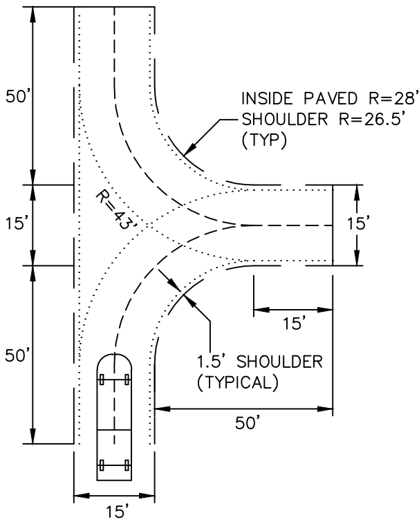
TYPE 1: HAMMERHEAD TURN AROUND
